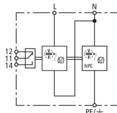
Basic circuit diagram DSH TT 2P 255 FM
