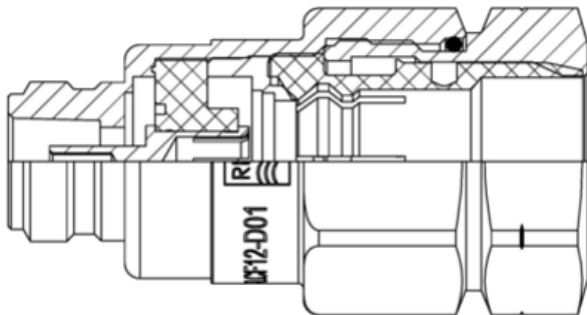
Cut NF-LCF12-D01_DRW.PNG
