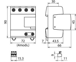
Dimension drawing DVA M NG 3P 100 FM
