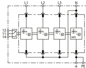
Basic circuit diagram DVA M NG 3P 100 FM
