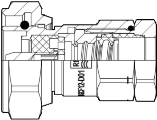
716M-SCF12-D01_DRW.png
