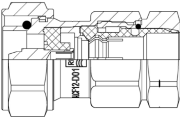
Cut 716M-LCF12-D01_DRW.PNG
