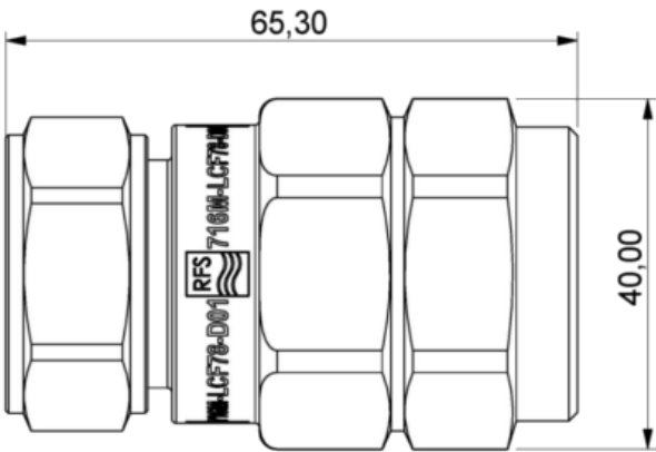
View 716M-LCF78-D01_DRW.PNG
