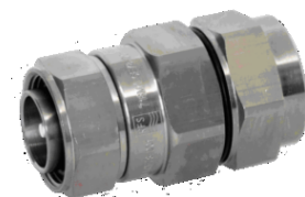
OMNI FIT™ Premium Connectors
