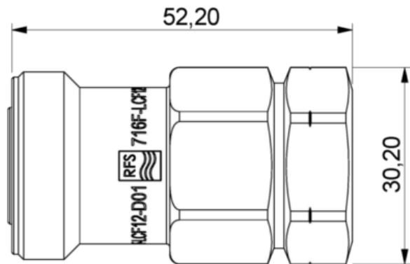
View 716F-LCF12-D01_DRW.PNG
