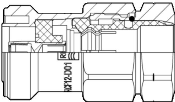
Cut 716F-LCF12-D01_DRW.PNG
