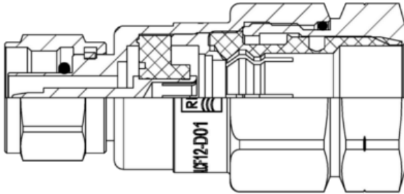
Cut NM-LCF12-D01_DRW.PNG
