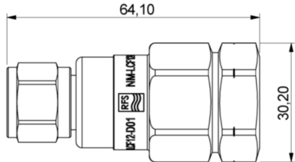
View NM-LCF12-D01_DRW.PNG
